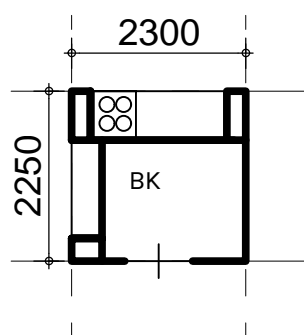
Comfort Cabin - samengestelde unit
